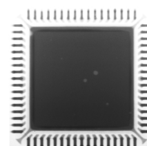
AMP One Voiding <3% Void Area
