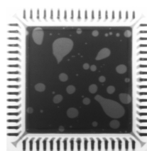
Typical Voiding 20% Void Area
